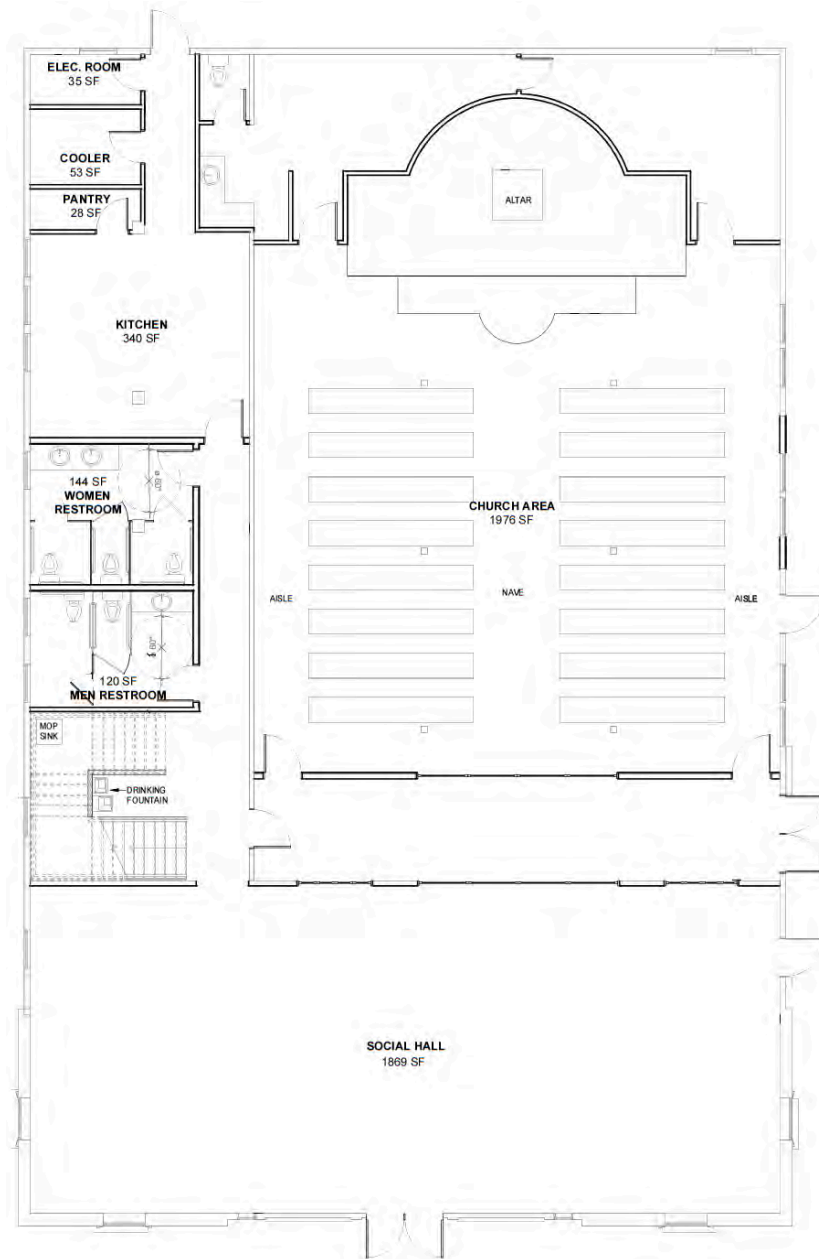
Preliminary First Floor Plans
